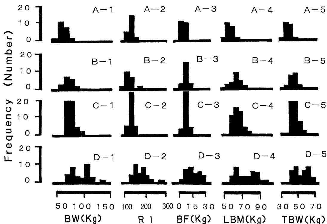
Fig. 1. Histogram of anthropometric index and body composition of the four groups.
