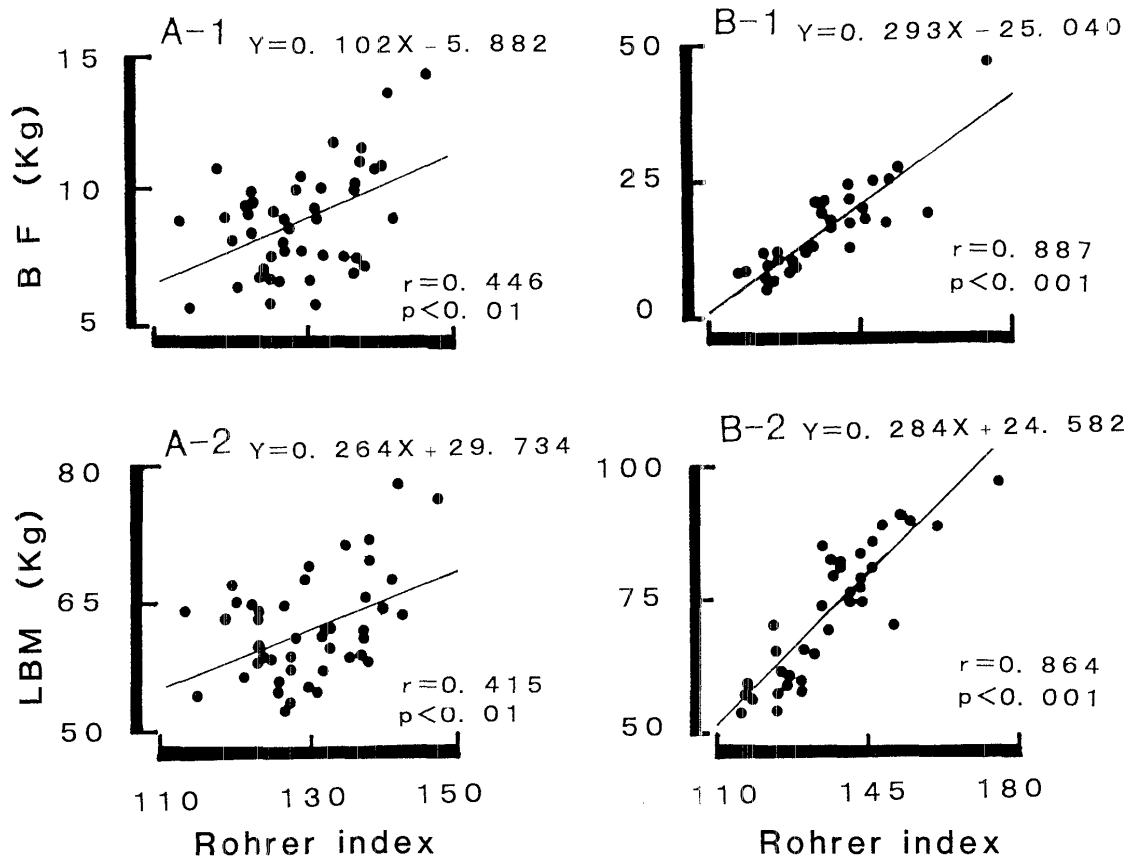
Fig. 2. Correlation coefficients, regression equation, and regression line between Rohrer index (RI) and body fat (BF), and between Rohrer index (RI) and lean body mass (LBM) for athletes of judo : baseball.
