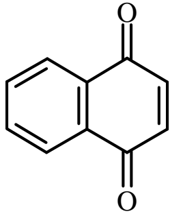
1,4-Naphthoquinone
