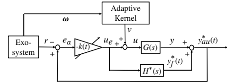
Fig. 2. Block Diagram of the ideal control system
