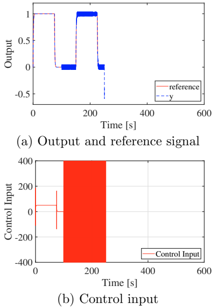
Fig. 4. Results with the previous adaptive PFC method: output and reference signal
