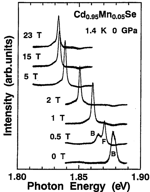
FIG. 1. Photoluminescence spectra in \text{Cd}_{0.95}\text{Mn}_{0.05}\text{Se} under various magnetic fields at 1.4 K and 0 GPa. The magnetic field is applied parallel to the c axis of the crystal. The features denoted as B and F are due to bound and free excitons, respectively.
