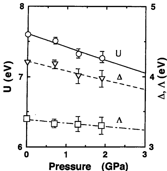
FIG. 5. Pressure dependencies of U ( \circ ), \Delta ( \nabla ), and \Lambda ( \square ) in \text{Cd}_{0.95}\text{Mn}_{0.05}\text{Se} . The solid, dashed, and dot-dashed lines are the linear fits to the experimental data of U , \Delta , and \Lambda , respectively.
