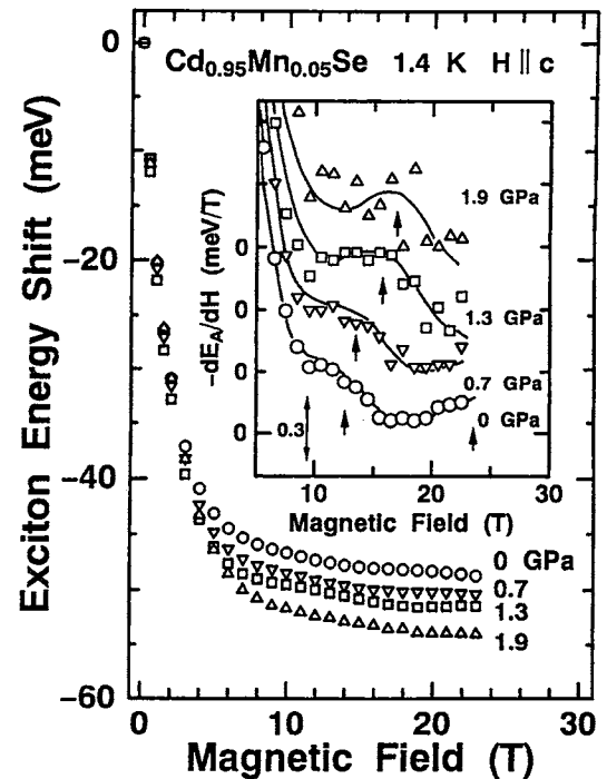
FIG. 2. Energy shift of the free exciton line in \text{Cd}_{0.95}\text{Mn}_{0.05}\text{Se} induced by the external magnetic field under 0 ( \circ ), 0.7 ( \nabla ), 1.3 ( \square ), and 1.9 ( \triangle ) GPa at 1.4 K. The inset shows the derivative of the exciton energy with respect to the external magnetic field under 0 ( \circ ), 0.7 ( \nabla ), 1.3 ( \square ), and 1.9 ( \triangle ) GPa. Solid lines are guides for the eye. Arrows show the field positions H_1 and H_2 .
