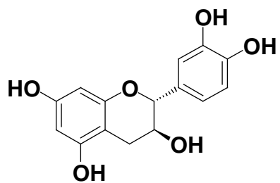
(A) (+)-Catechin
