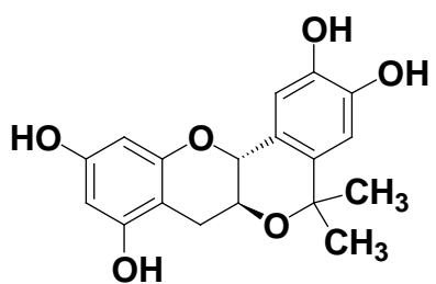
(B) Planar catechin analogue
