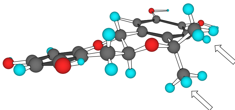
(B) Planar catechin analogue
