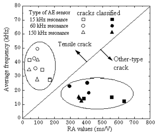
Fig. 2 Qualification of the damage by AE parameters.
