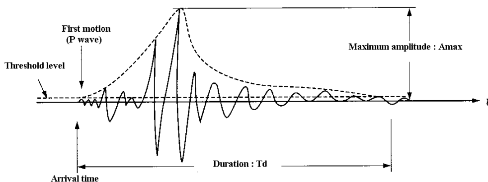
Fig. 1 AE waveform parameters.
