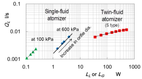
Figure 9. Comparison of mist generation rate between single-fluid type and twin-fluid type.
