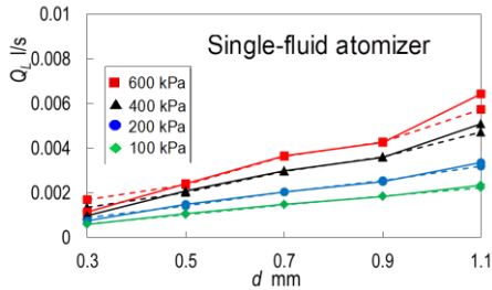
Figure 7. Mist flow rate against orifice diameter for single-fluid atomizer.
