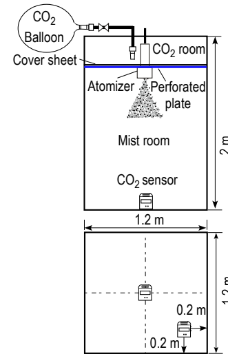
Figure 4. Test room for CO 2 adsorption by mist.
